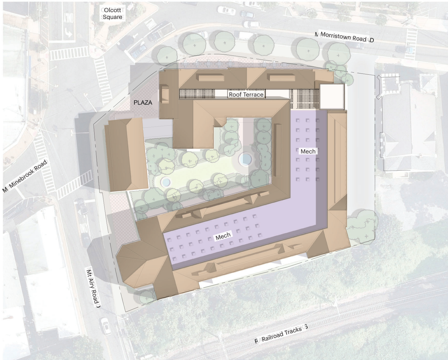
Roof Plan
